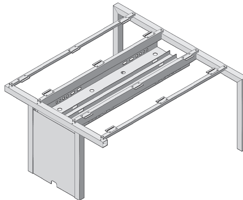
3D ESTRUTURA | 3D STRUCTURE | 3D ESTRUCTURA Mesa dupla | Double desk | Mesa doble
